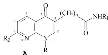
Figure 2. General structure of 1,8-naphthyridine derivatives.
