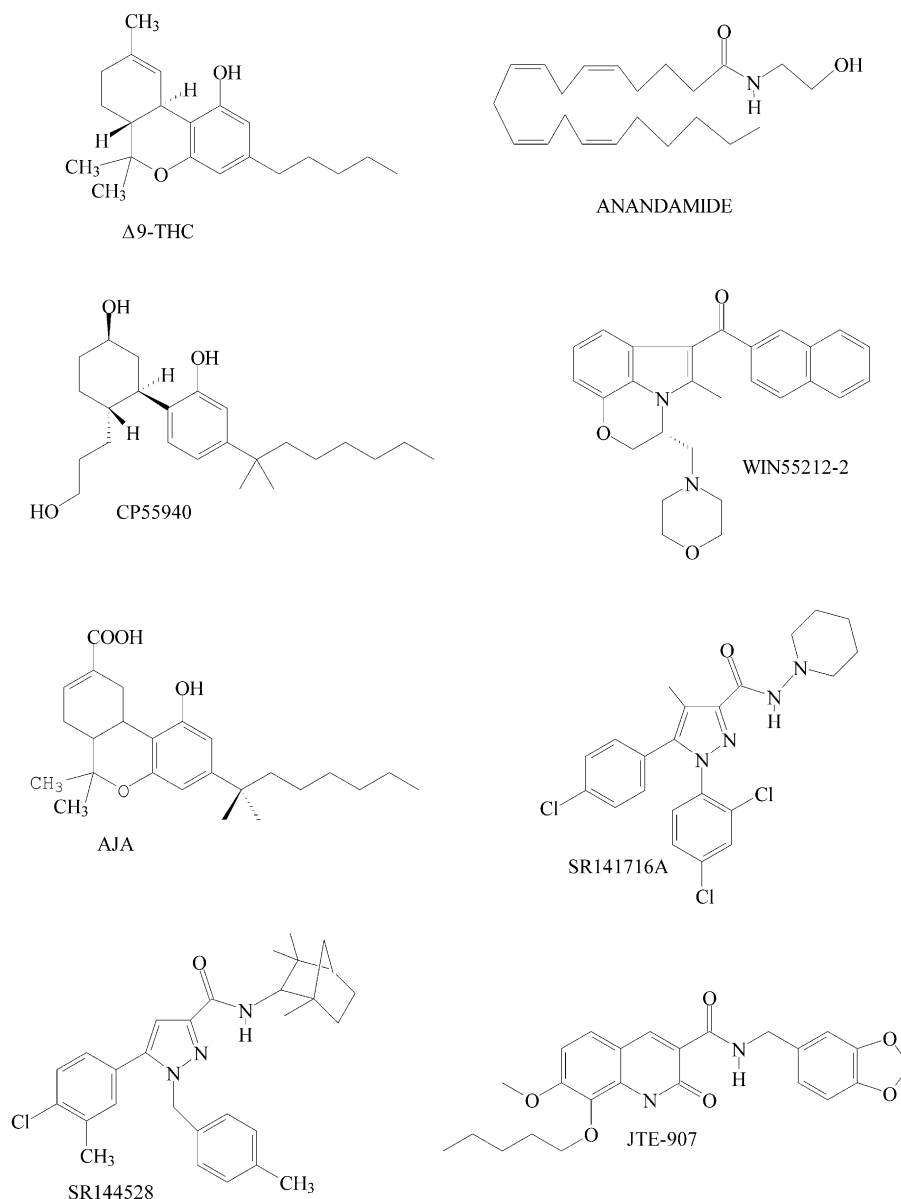
Figure 1. Molecular structures of cannabinoid CB 1 and CB 2 receptor ligands.
